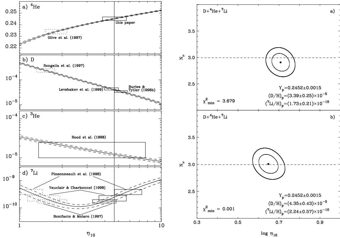
Figure 4: The abundance of (a) ^4\text{He} , (b) D, (c) ^3\text{He} and (d) ^7\text{Li} as a function of \eta_{10} \equiv 10^{10} \eta , where \eta is the baryon-to-photon number ratio, as given by the standard hot big bang nucleosynthesis model. The abundances of D, ^3\text{He} and ^7\text{Li} are number ratios relative to H. For ^4\text{He} , the mass fraction Y is shown. The value of Izotov & Thuan (1998) and Izotov et al. (1999) Y_p = 0.245 \pm 0.002 gives \eta = (4.7^{+1.0}_{-0.8}) \times 10^{-10} as shown by the solid vertical line. We show other data with 1\sigma boxes.
