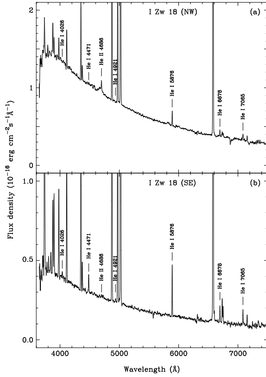
Figure 2: Spectra of the brightest parts of the NW and the SE components of I Zw 18. The positions of He I lines used for ^4\text{He} abundance determination are marked. Note the effect of underlying stellar absorption is much larger in the NW than in the SE component: all marked He I lines in the spectrum of the SE component are in emission while the two He I \lambda 4026 and \lambda 4921 lines are in absorption and the He I \lambda 4471 emission line is barely detected in the spectrum of the NW component.
