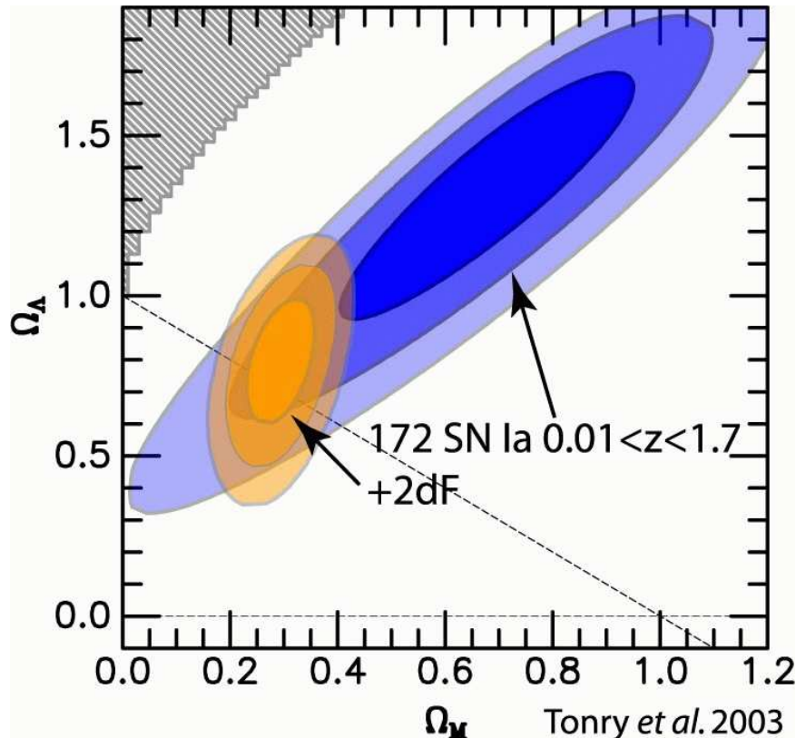
Figure 1.1: This shows the preferred region in the \Omega_m - \Omega_\Lambda plane from a study of 172 supernovae, and also how the constraints tighten when the 2dF galaxy redshift survey power spectrum is added as an additional constraint. [Reproduced with permission from Tonry et al. [16]. ]
